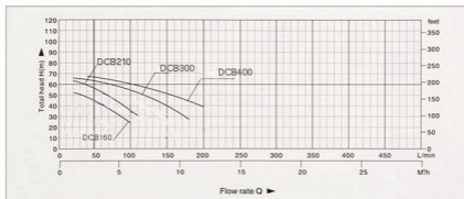
PERFORMANCE CHART AT n=2850RPM
